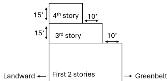
Figure 8-8B-5.3 Additional Stories Stepback
