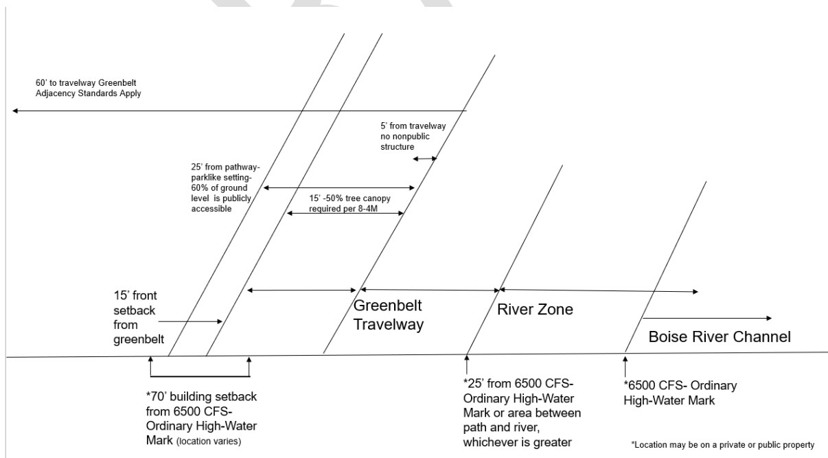
Figure 8-8B-5.4 Greenbelt Adjacency
