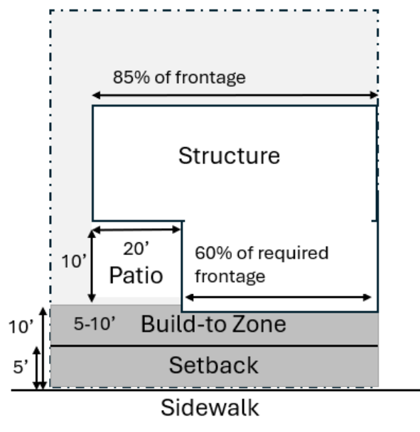
Figure 8-8B-5.2 Build-To Street Relationship
